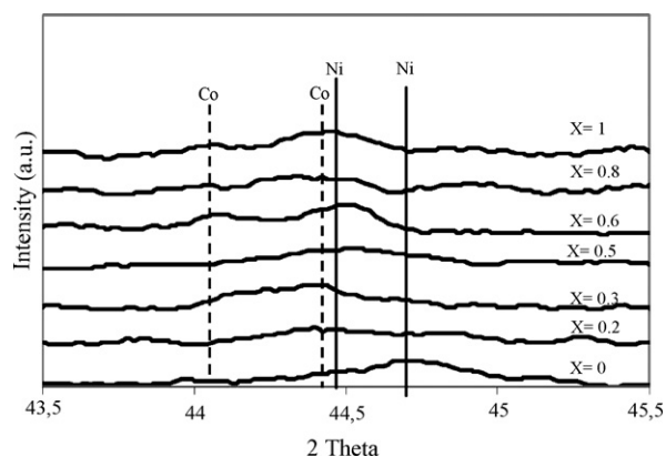
Fig. 8. XRD patterns of peaks respect to \text{Ni}^0 and \text{Co}^0 phases of \text{LaNi}_{1-x}\text{Co}_x\text{O}_3 .
