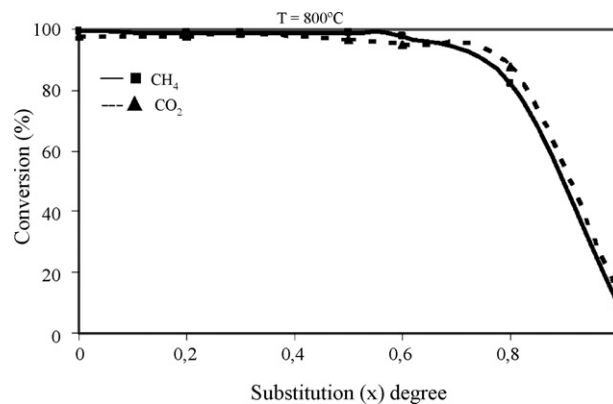
Fig. 10. \text{CH}_4 and \text{CO}_2 conversions on unreduced \text{LaNi}_{1-x}\text{Co}_x\text{O}_3 at 800 °C.
